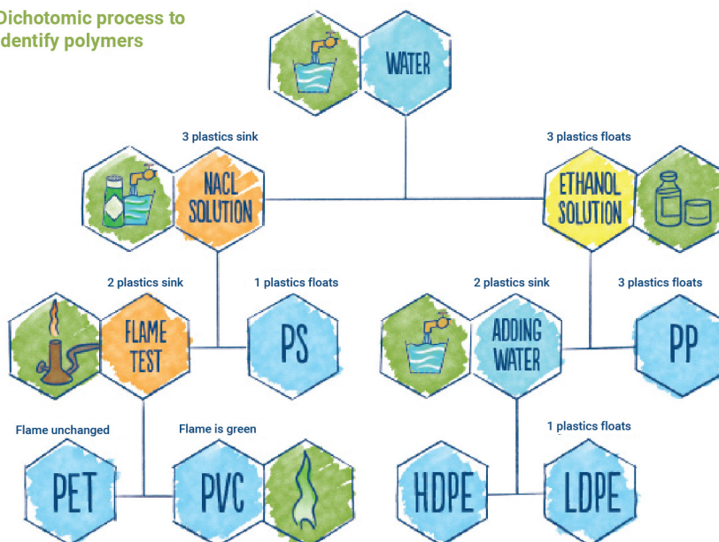
Infographic 2.4.3: Dichotomic process to identify polymers
